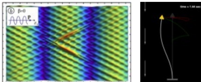
From left to right: A wave impinging two shear bands; flutter of an elastic rod
