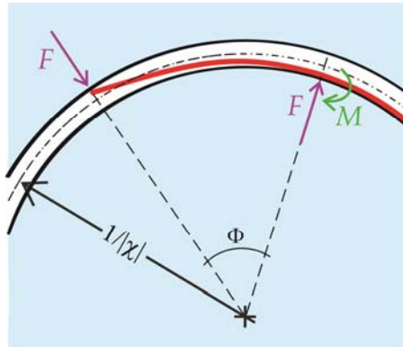
Fig 2: Micromechanics of an elastic rod inside a frictionless rigid channel that shows the reactions developing at the contact points
