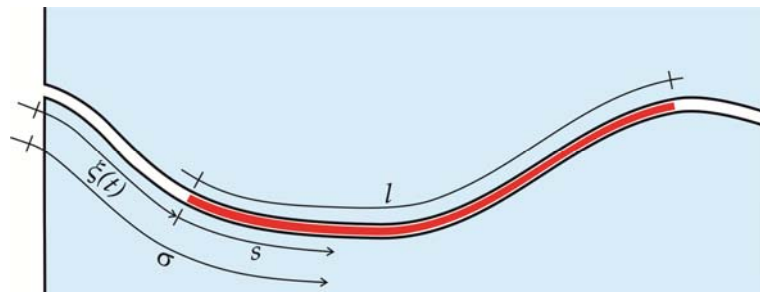
Fig.1: An extensible elastic rod (rectilinear in its undeformed configuration) of length l within a smooth curvilinear channel. Its configuration is defined by the evolution in time of the curvilinear coordinate \xi(t) .
